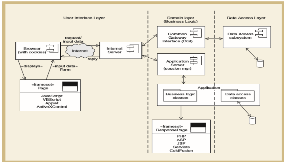
Figure 3.1: Component Diagram of <Name of the System>
